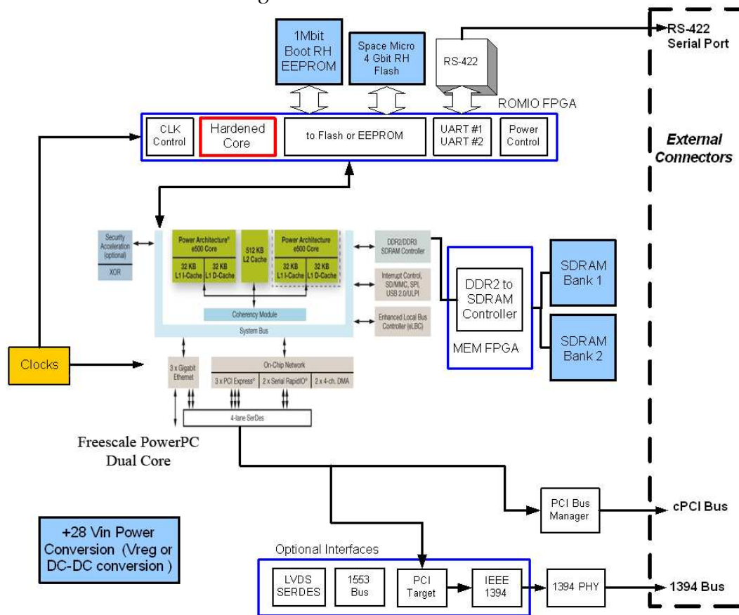
Proton400k-L™ Block Diagram
